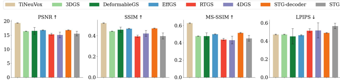
Figure 3.9: Quantitative comparison of all methods evaluated on the strictly-monocular iPhone dataset. Figure taken from Liang et al., 2025 .
