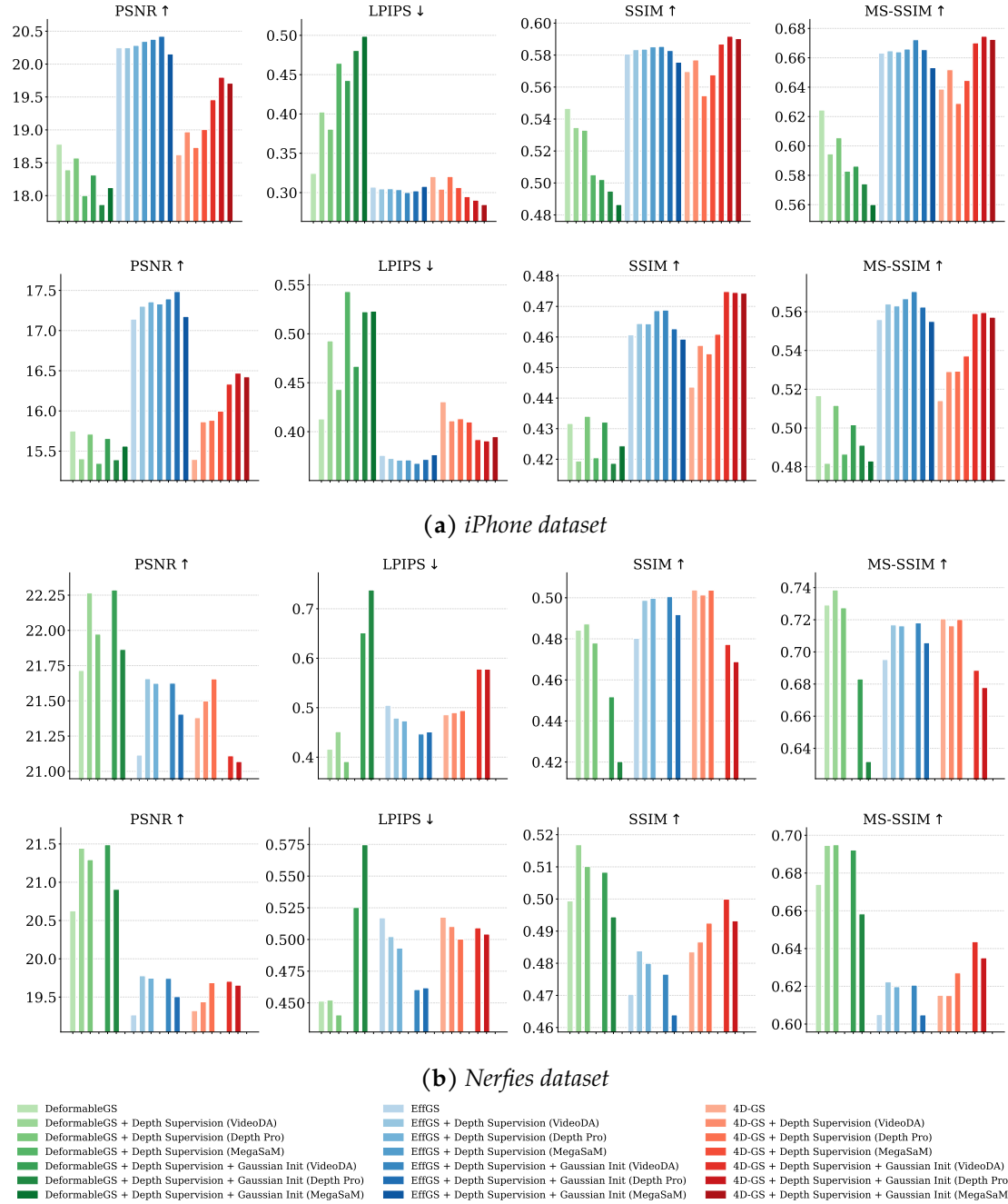
Figure 5.15: All metrics for (a) iPhone and (b) Nerfies, reported for the full image (top) and the foreground region (bottom). The results highlight that the effect of depth-based supervision varies substantially across methods and datasets. Furthermore, improvements on the dynamic foreground are generally not larger than those measured on the full image.
